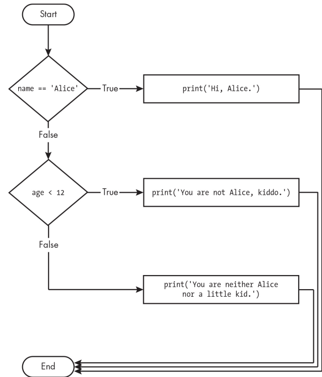
Figure 2-7: The flowchart for the littleKid.py program Description
