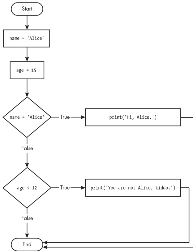
Figure 2-4: The flowchart for an elif statement Description
