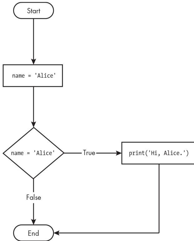
Figure 2-2: The flowchart for an if statement Description
