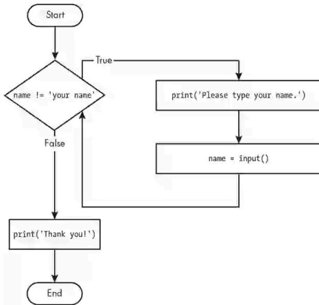
Figure 3-3: The flowchart for the yourName.py program
