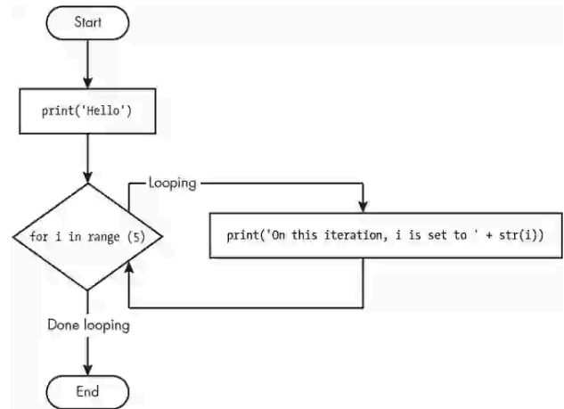
Figure 3-6: The flowchart for the fiveTimes.py program Description
